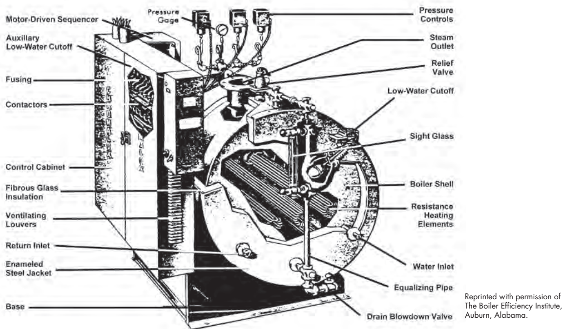
Figure 9.2.3. Electric boiler
