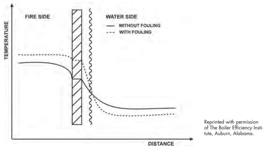
Figure 9.2.5. Effect of fouling on water side
